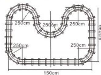
Track diagram of the chase car
